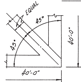
CORNER DETAIL C
