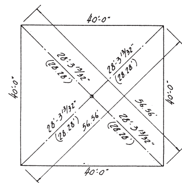
40' SQUARE DIMENSIONING
